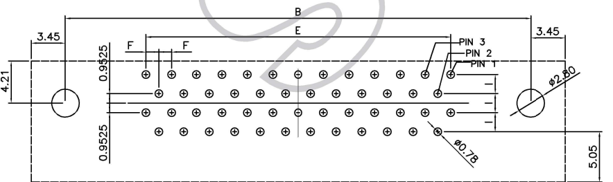
Recommended PCB Layout Layout Tolerance±0.05mm
