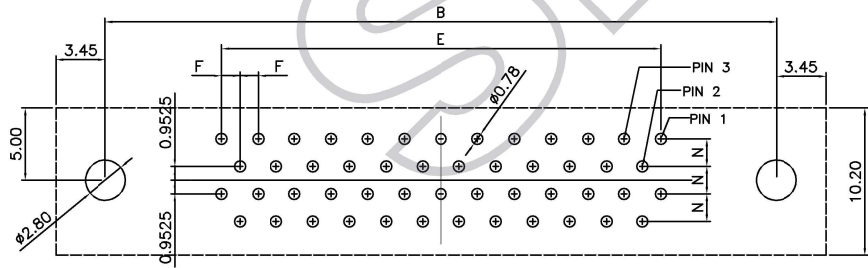
Recommended PCB Layout Layout Tolerance±0.05mm
