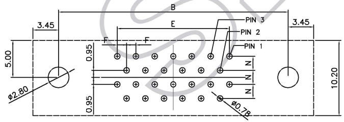
Recommended PCB Layout Layout Tolerance±0.05mm
