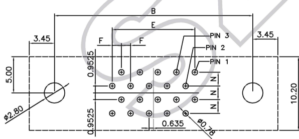
Recommended PCB Layout Layout Tolerance \pm 0.05\text{mm}
