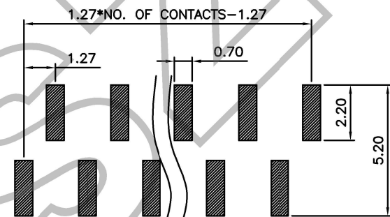
Recommended PCB Layout Layout Tolerance ±0.05mm
