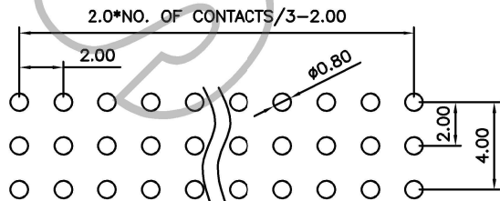
Recommended PCB Layout Layout Tolerance ±0.05mm
