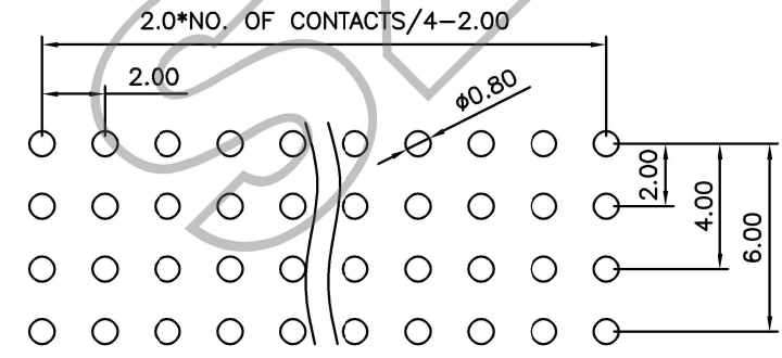
Recommended PCB Layout Layout Tolerance ±0.05mm
